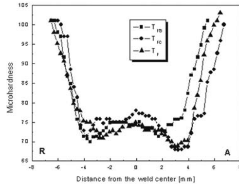
Fig. 8. Horizontal hardness ( \text{HV}_{0.1} ) profile across friction stir welds, “A” means advancing side, “R” retreating side.
